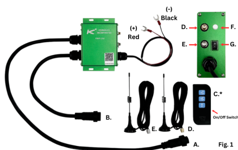
Fig. 1 A. Connect to handheld control B. Connect to HPU C. Key fob* D. Bluetooth Antenna (Gold) E. RF Antenna (Silver) F. Key fob Pairing Button G. Power ON/OFF
