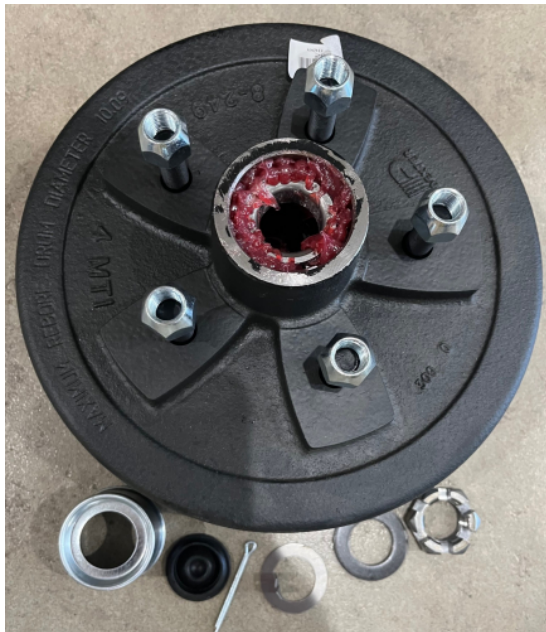
DEXTER 3500# Axle Trailer Brake Drum with 5on4.5" Bolt Pattern
